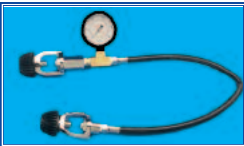
AA68 Tank to tank equalizer with bleeder valve and 5000psi gauge
